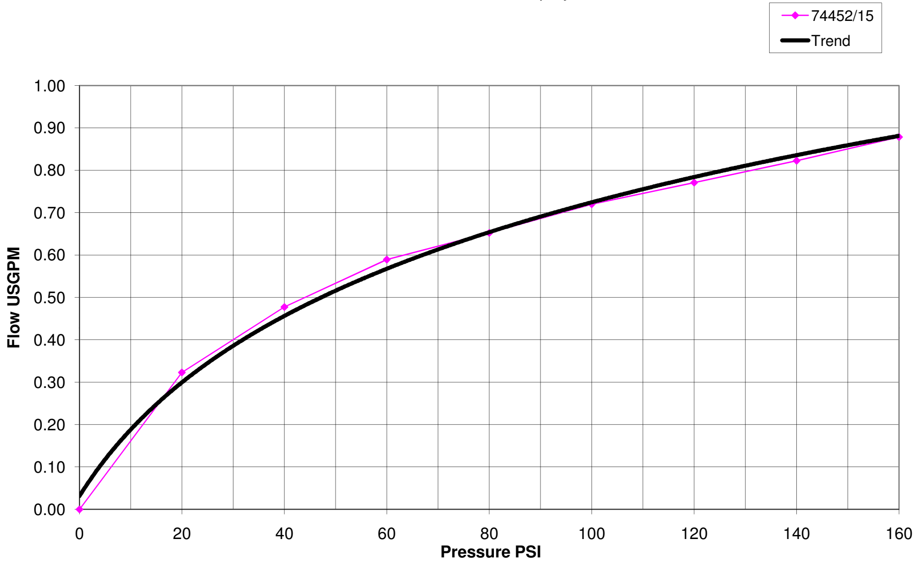
Flow Chart for 74452/15 J35 Spray in USGPM
